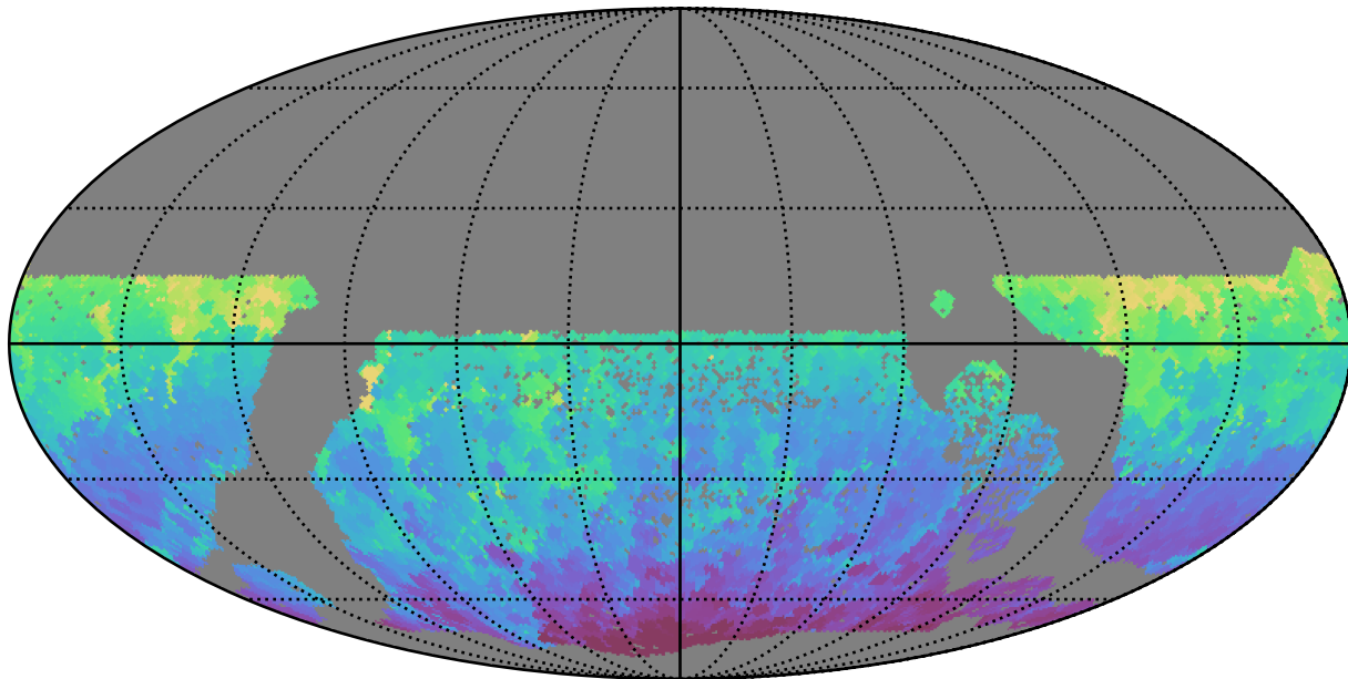
too_elab_r256_d3_giz_v3.4_10yrs WFD i band: Min HA
