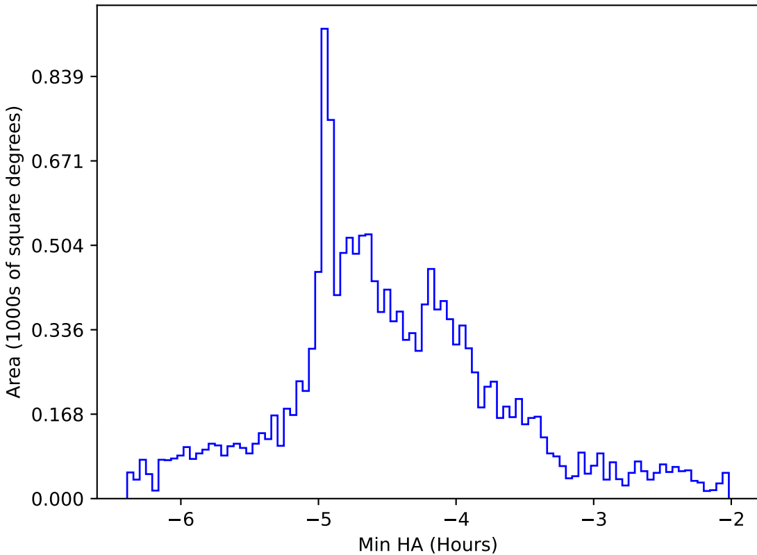
too_elab_r256_d3_giz_v3.4_10yrs WFD g band: Min HA
