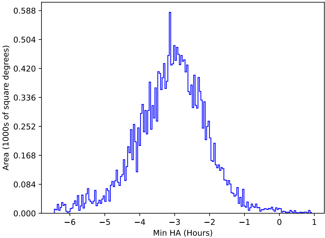
too_elab_r256_d3_giz_v3.4_10yrs All sky u band: Min HA
