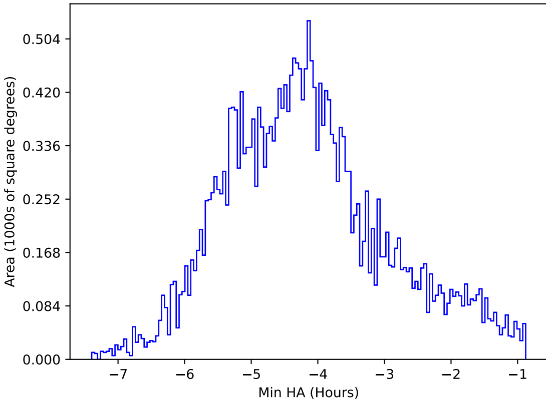
too_elab_r256_d3_giz_v3.4_10yrs All sky r band: Min HA
