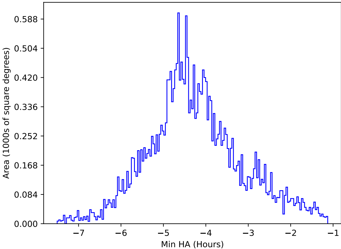
too_elab_r256_d3_giz_v3.4_10yrs All sky i band: Min HA
