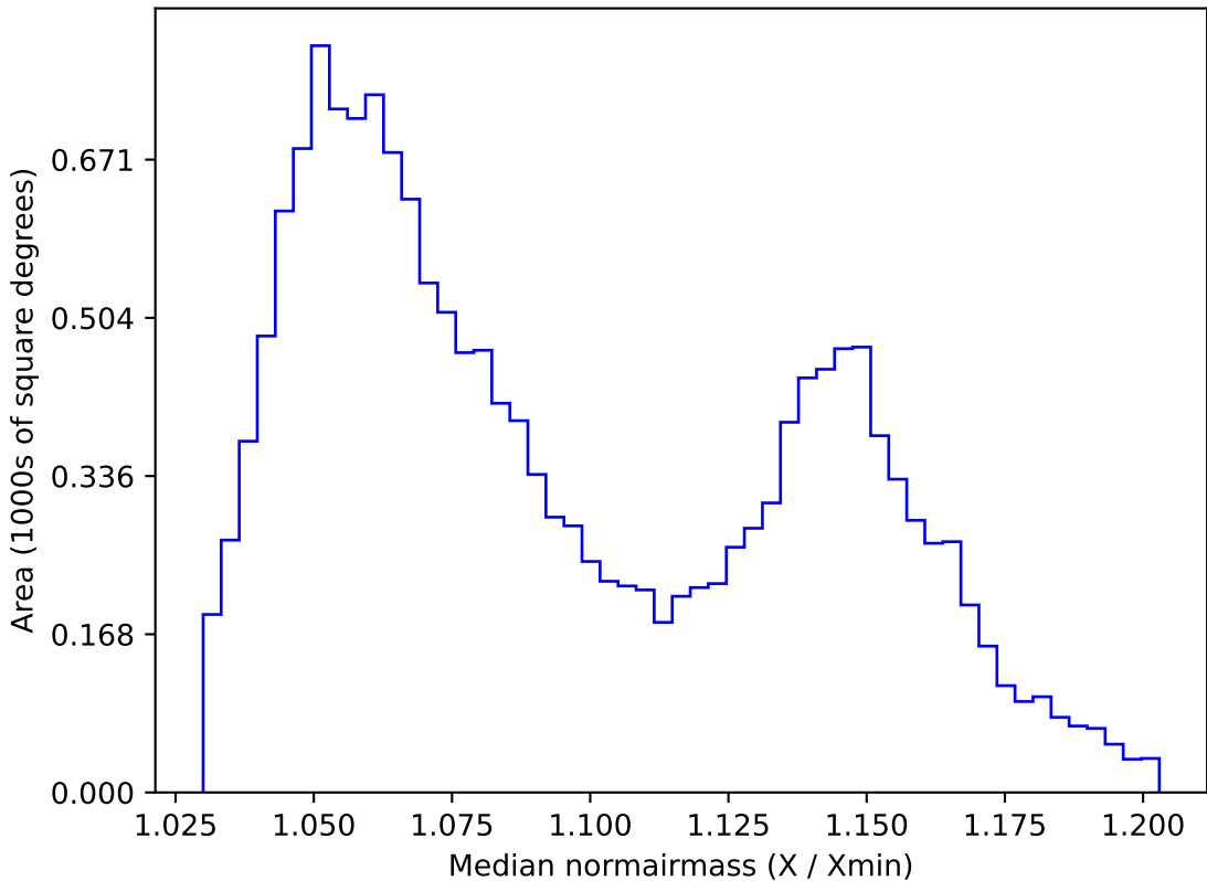
too_elab_r256_d3_giz_v3.4_10yrs WFD y band: Median normairmass
