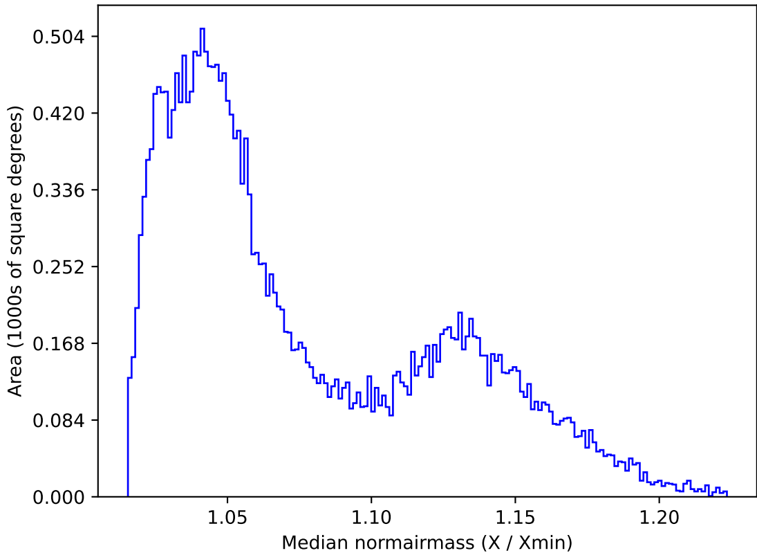
too_elab_r256_d3_giz_v3.4_10yrs All sky r band: Median normairmass
