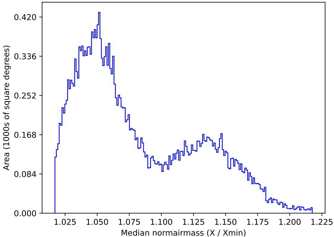
too_elab_r256_d3_giz_v3.4_10yrs All sky i band: Median normairmass
