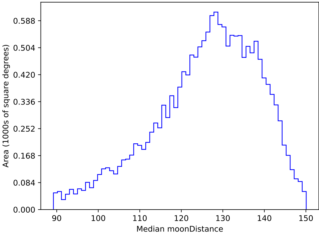
too_elab_r256_d3_giz_v3.4_10yrs WFD u band: Median moonDistance
