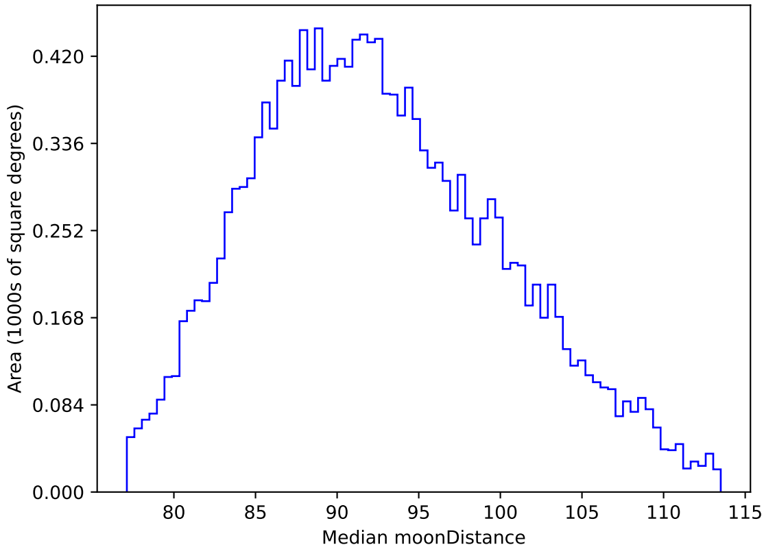
too_elab_r256_d3_giz_v3.4_10yrs WFD i band: Median moonDistance
