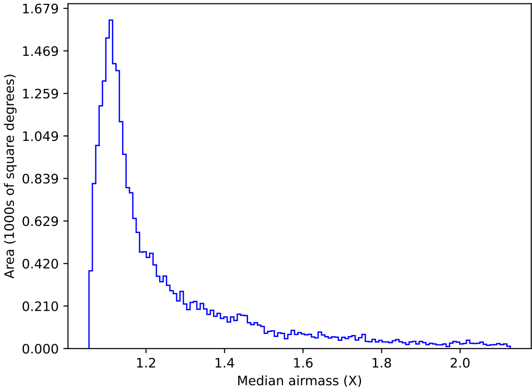
too_elab_r256_d3_giz_v3.4_10yrs Yr 1 r band: Median airmass
