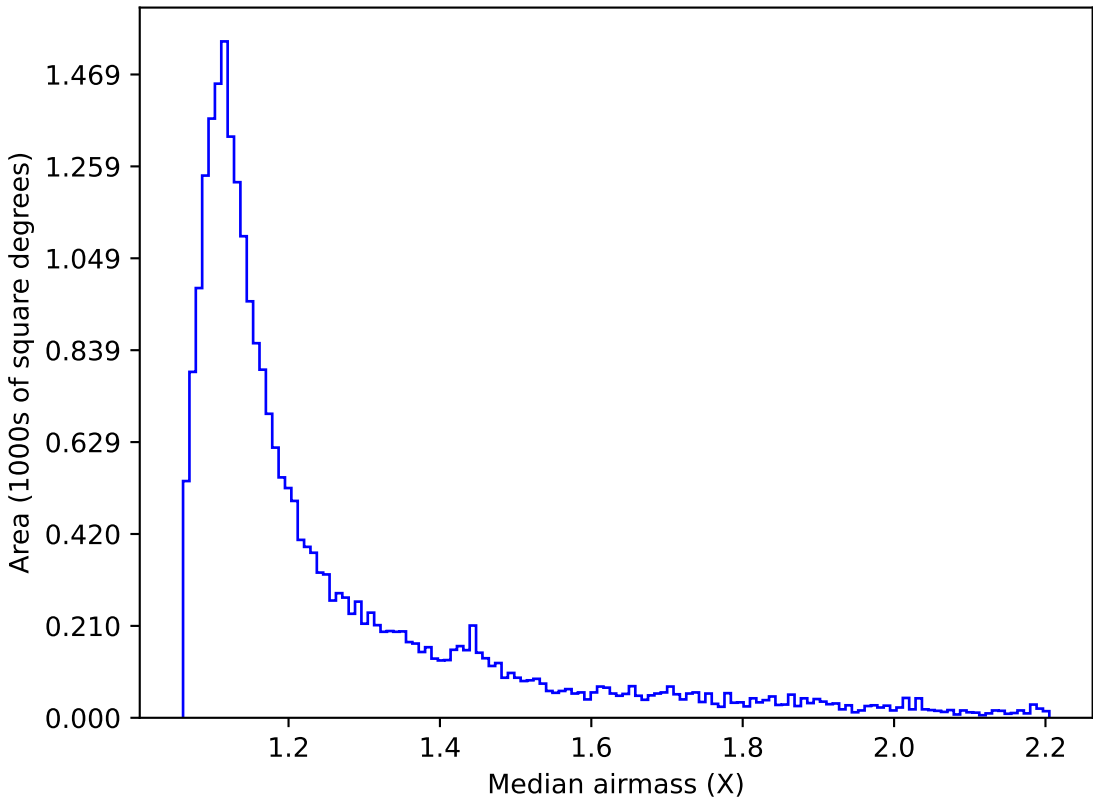
too_elab_r256_d3_giz_v3.4_10yrs Yr 1 i band: Median airmass
