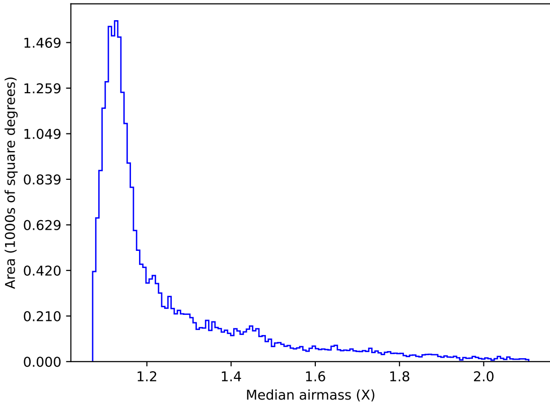
too_elab_r256_d3_giz_v3.4_10yrs Yr 1 all bands: Median airmass
