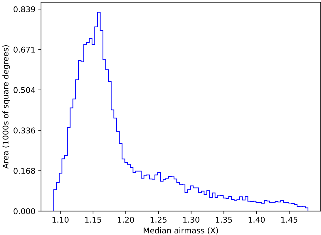
too_elab_r256_d3_giz_v3.4_10yrs WFD z band: Median airmass
