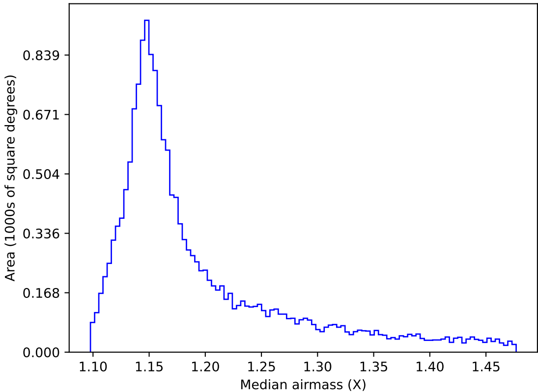
too_elab_r256_d3_giz_v3.4_10yrs WFD y band: Median airmass
