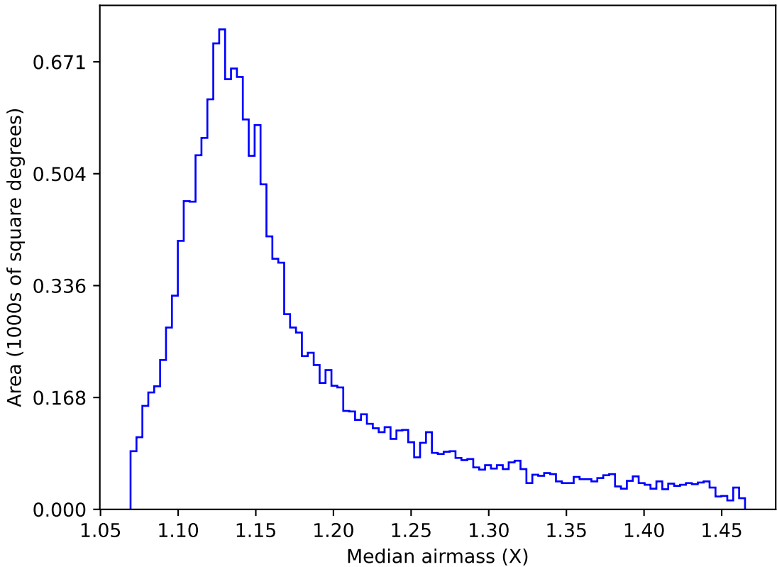
too_elab_r256_d3_giz_v3.4_10yrs WFD u band: Median airmass
