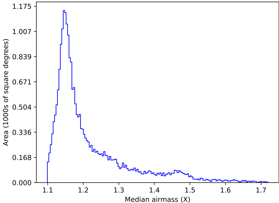
too_elab_r256_d3_giz_v3.4_10yrs All sky y band: Median airmass
