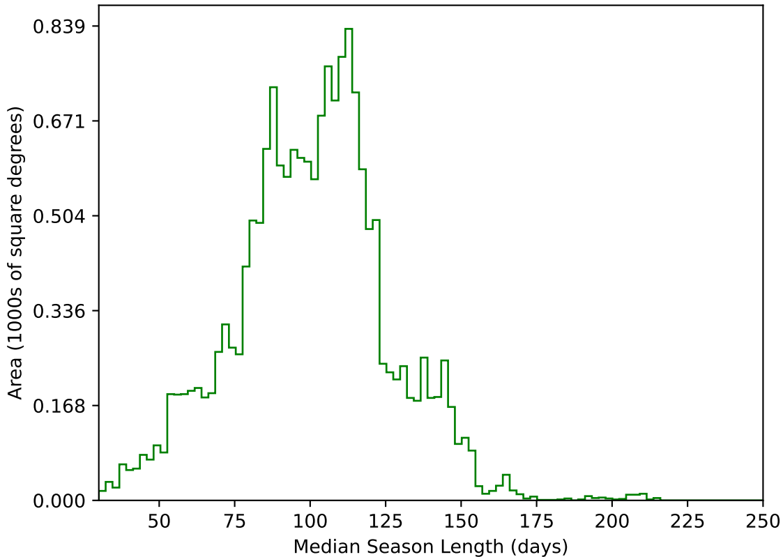
too_elab_r256_d3_giz_v3.4_10yrs WFD g band: Median Season Length
