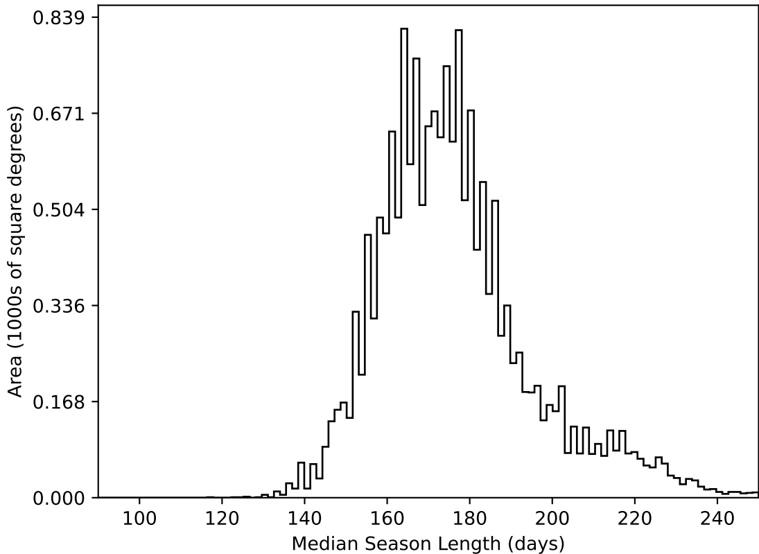
too_elab_r256_d3_giz_v3.4_10yrs WFD all bands: Median Season Length
