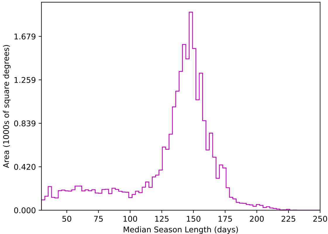
too_elab_r256_d3_giz_v3.4_10yrs All sky z band: Median Season Length
