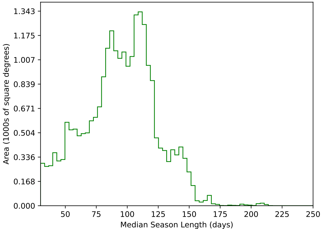
too_elab_r256_d3_giz_v3.4_10yrs All sky g band: Median Season Length
