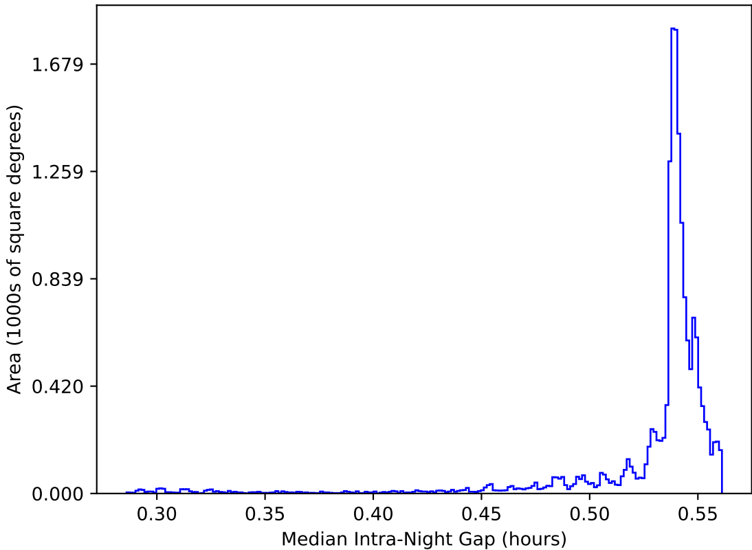
too_elab_r256_d3_giz_v3.4_10yrs WFD: Median Intra-Night Gap
