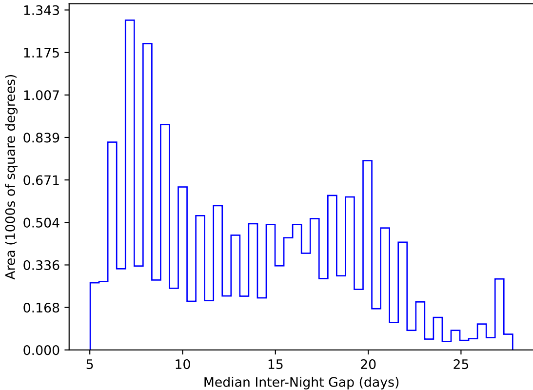
too_elab_r256_d3_giz_v3.4_10yrs WFD y band: Median Inter-Night Gap
