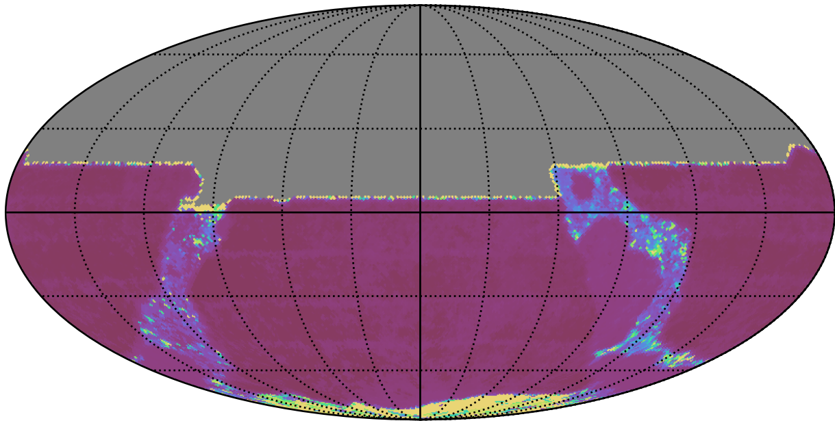
too_elab_r256_d3_giz_v3.4_10yrs All sky y band: Median Inter-Night Gap
