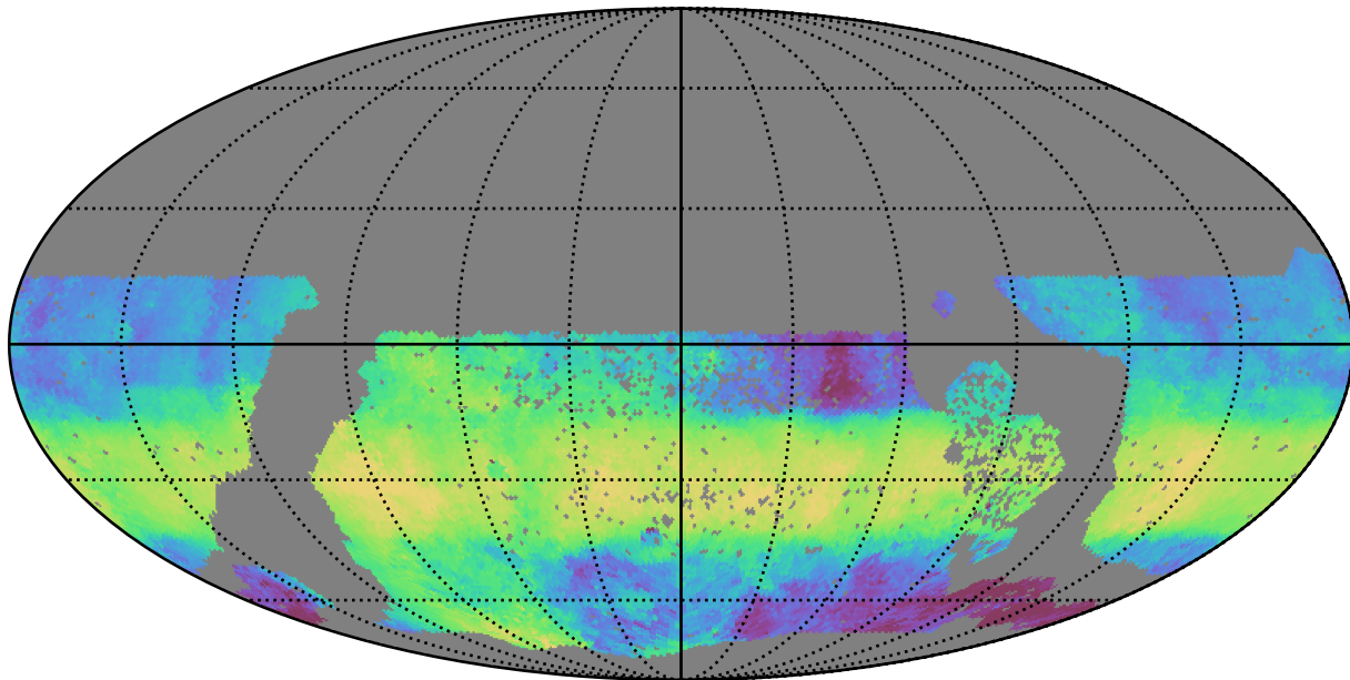
too_elab_r256_d3_giz_v3.4_10yrs WFD z band: Median HA
