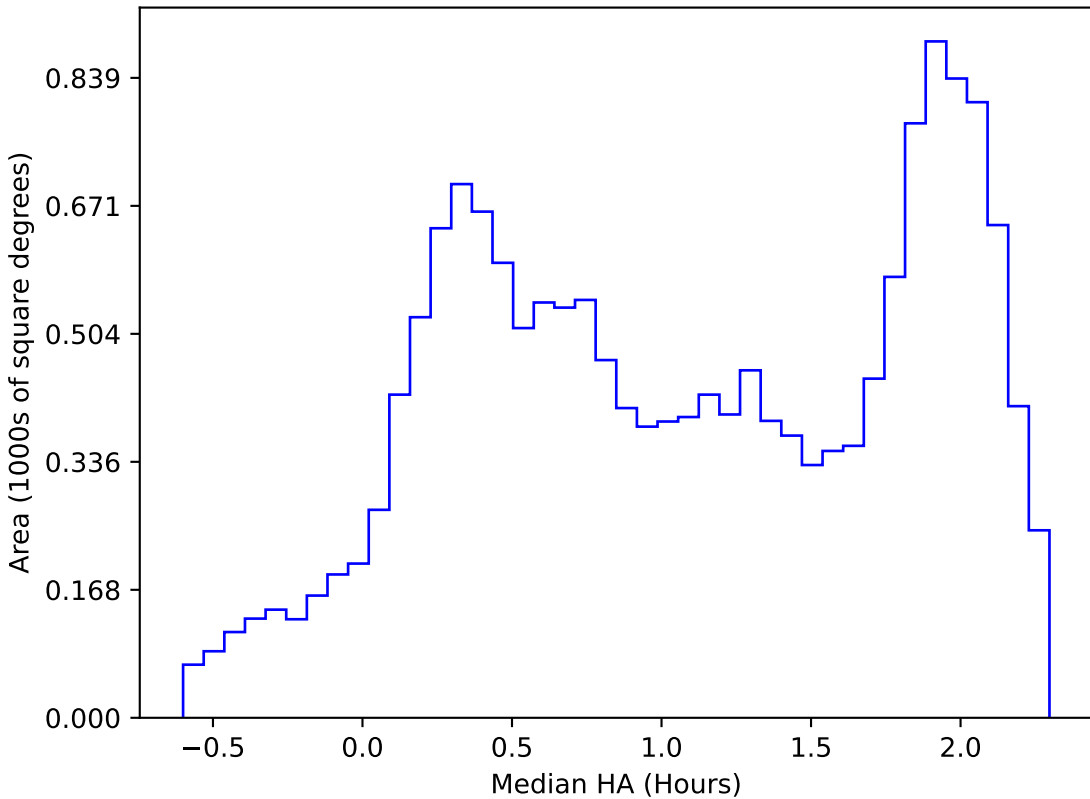
too_elab_r256_d3_giz_v3.4_10yrs WFD i band: Median HA
