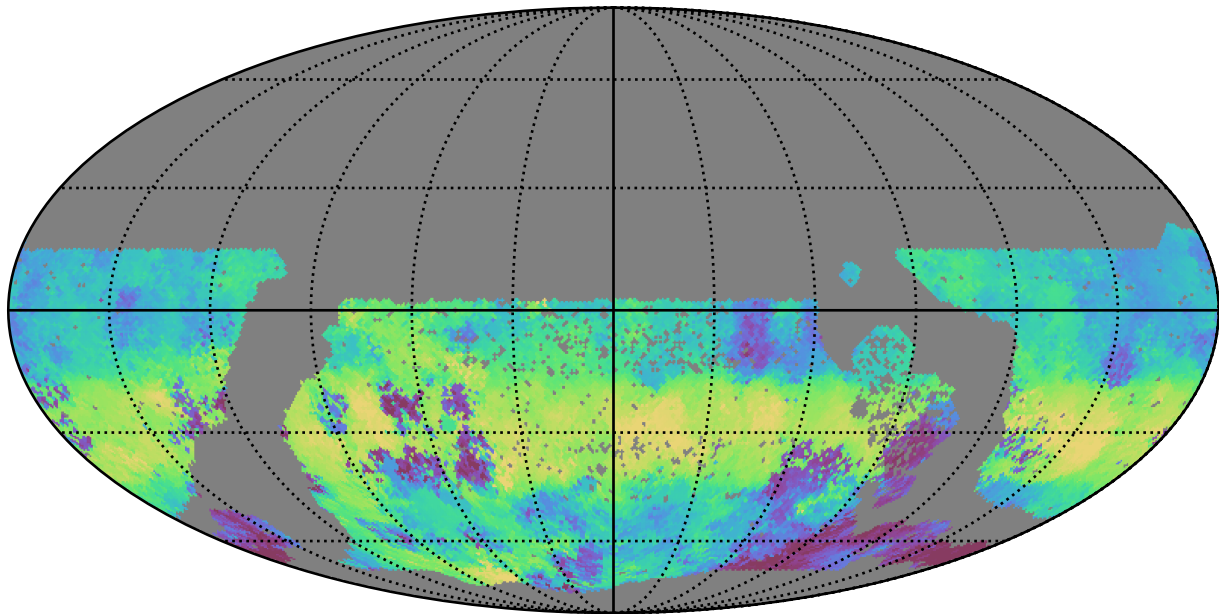
too_elab_r256_d3_giz_v3.4_10yrs WFD g band: Median HA
