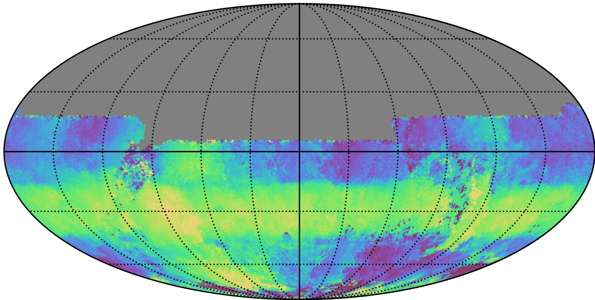
too_elab_r256_d3_giz_v3.4_10yrs All sky u band: Median HA
