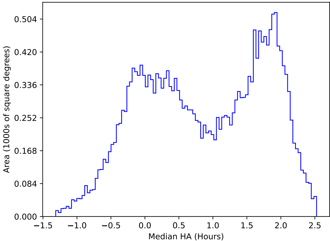
too_elab_r256_d3_giz_v3.4_10yrs All sky u band: Median HA
