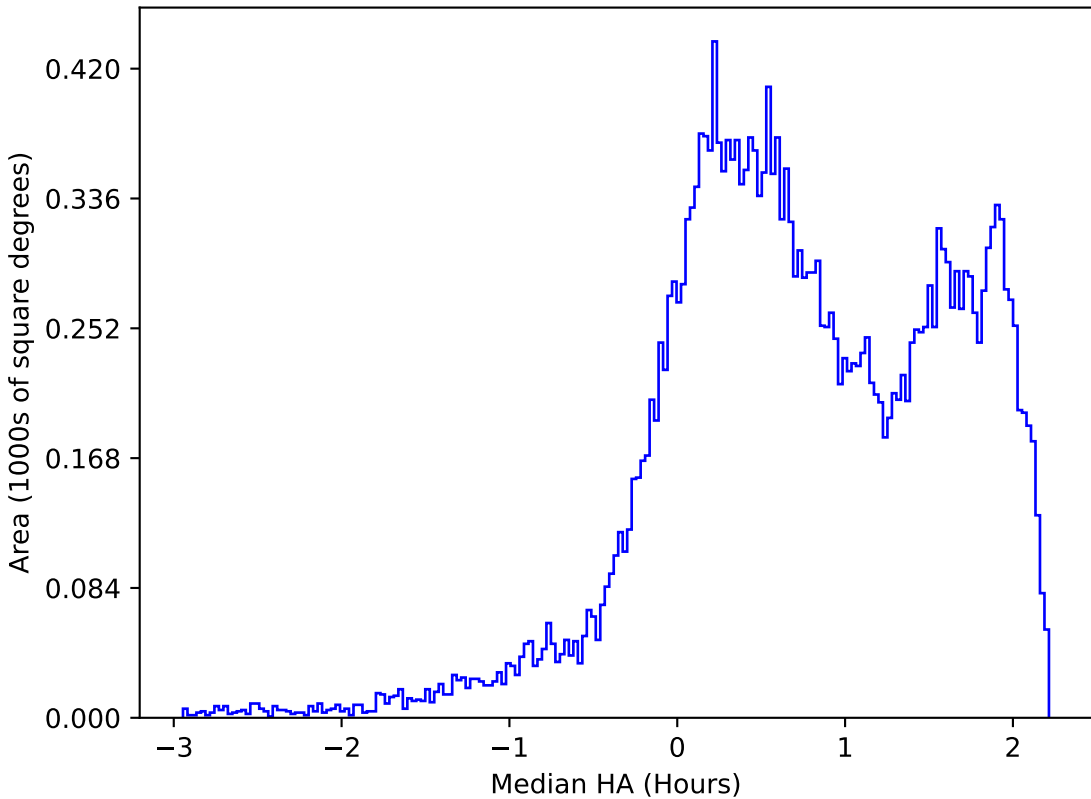
too_elab_r256_d3_giz_v3.4_10yrs All sky r band: Median HA
