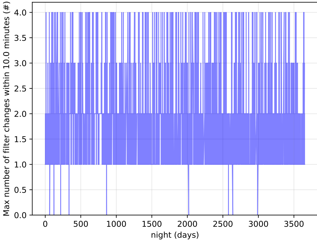
too_elab_r256_d3_giz_v3.4_10yrs Per Night: Max number of filter changes within 10.0 minutes
