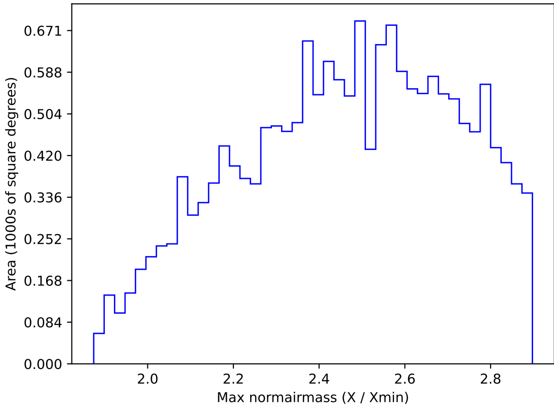
too_elab_r256_d3_giz_v3.4_10yrs WFD all bands: Max normairmass
