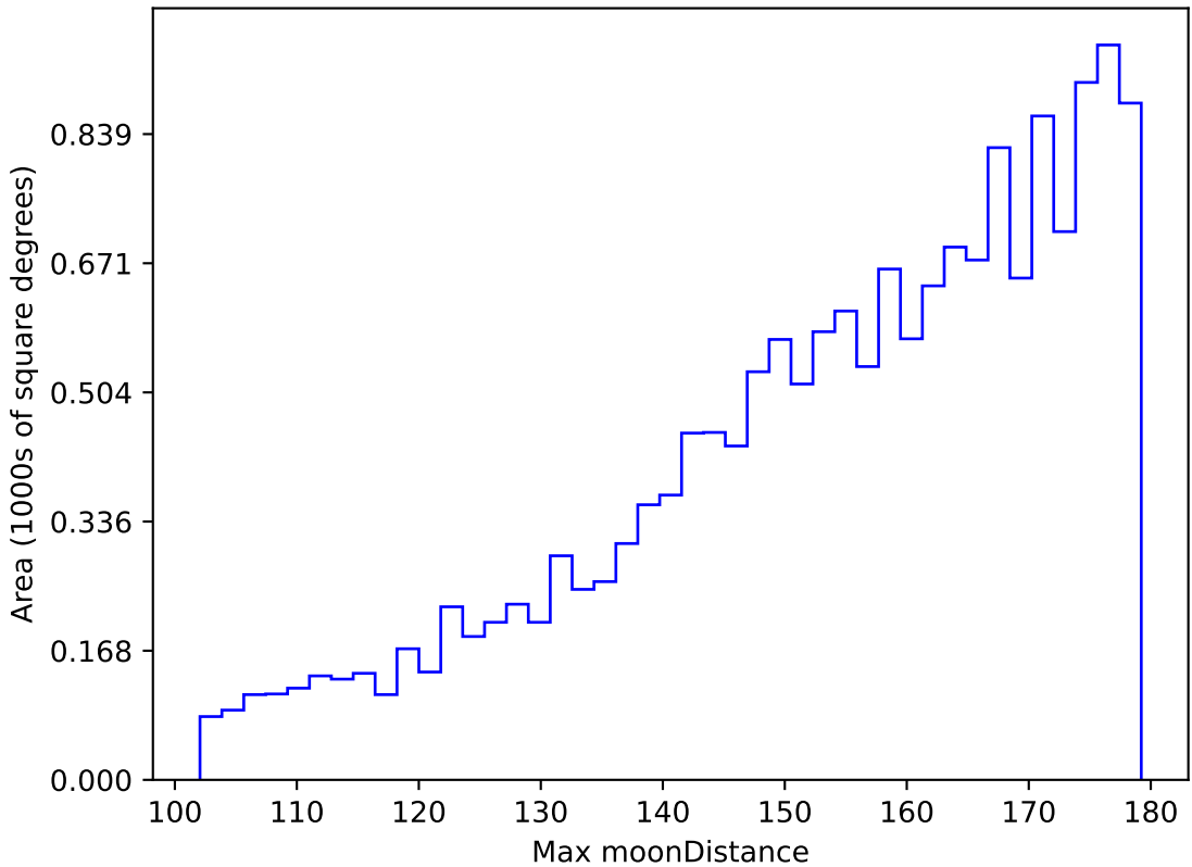
too_elab_r256_d3_giz_v3.4_10yrs WFD u band: Max moonDistance
