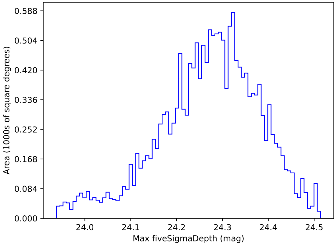
too_elab_r256_d3_giz_v3.4_10yrs WFD i band: Max fiveSigmaDepth
