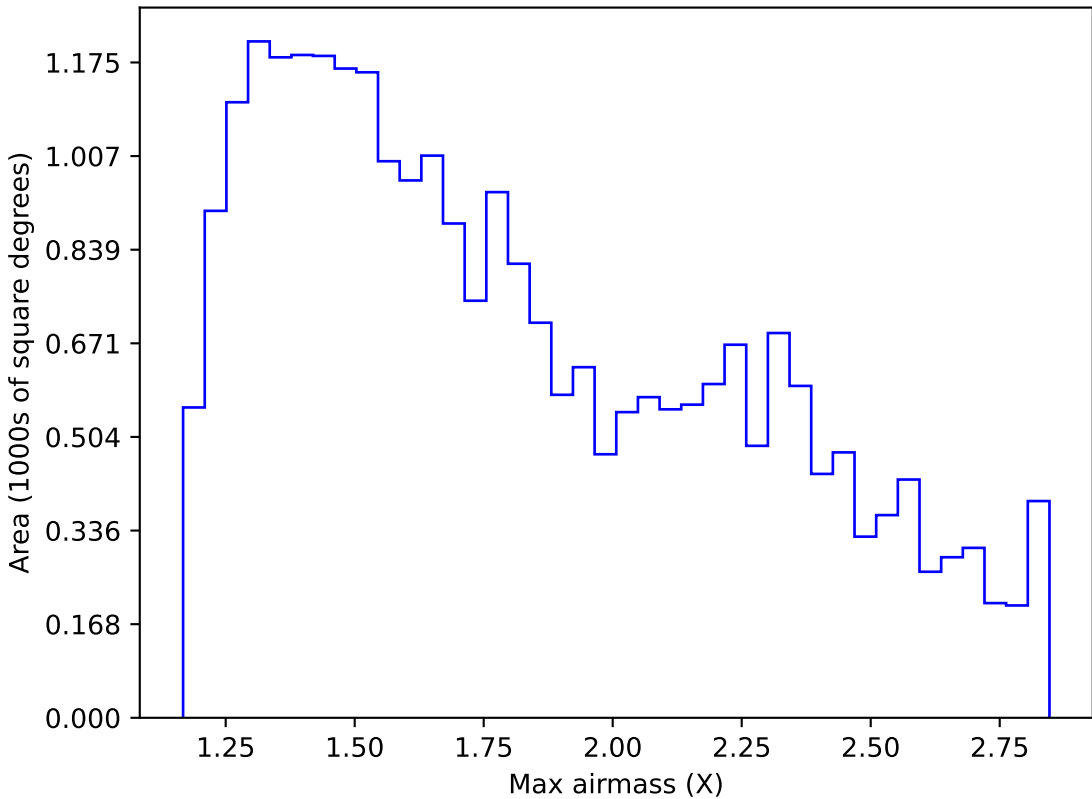
too_elab_r256_d3_giz_v3.4_10yrs Yr 1 i band: Max airmass
