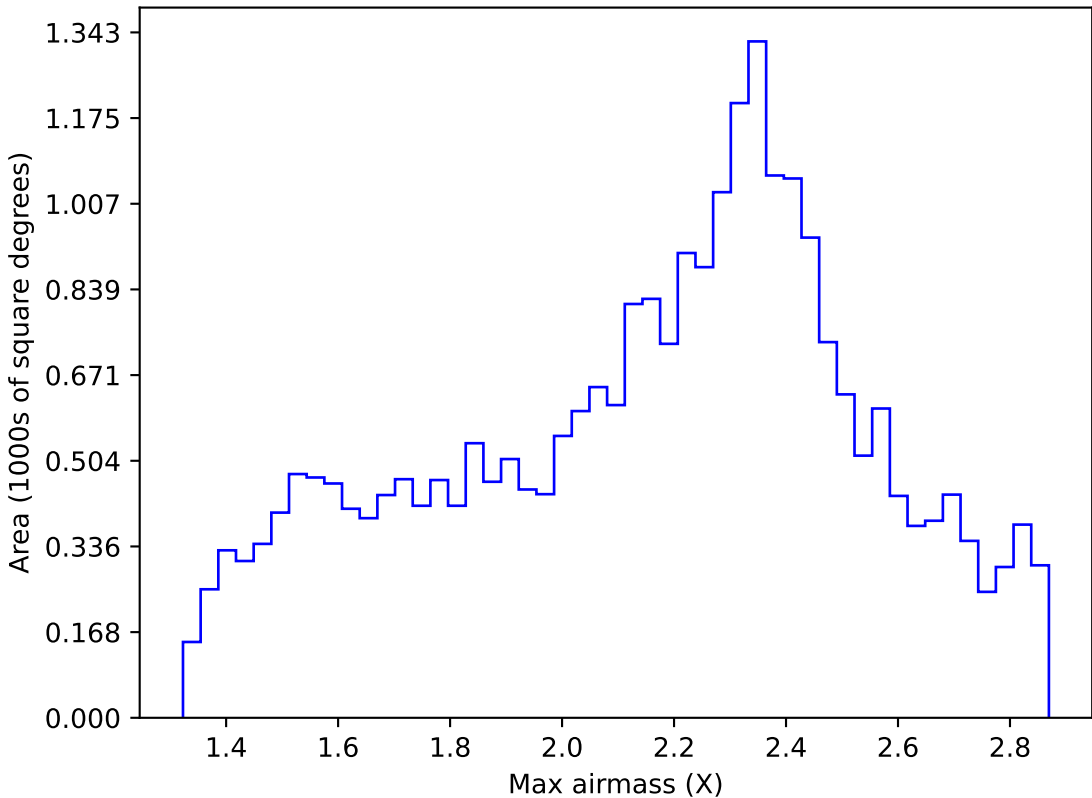
too_elab_r256_d3_giz_v3.4_10yrs Yr 1 all bands: Max airmass
