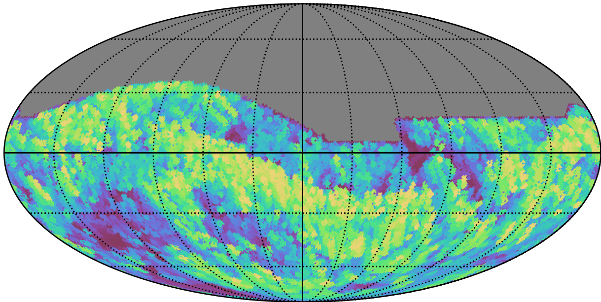
too_elab_r256_d3_giz_v3.4_10yrs All sky z band: Max airmass
