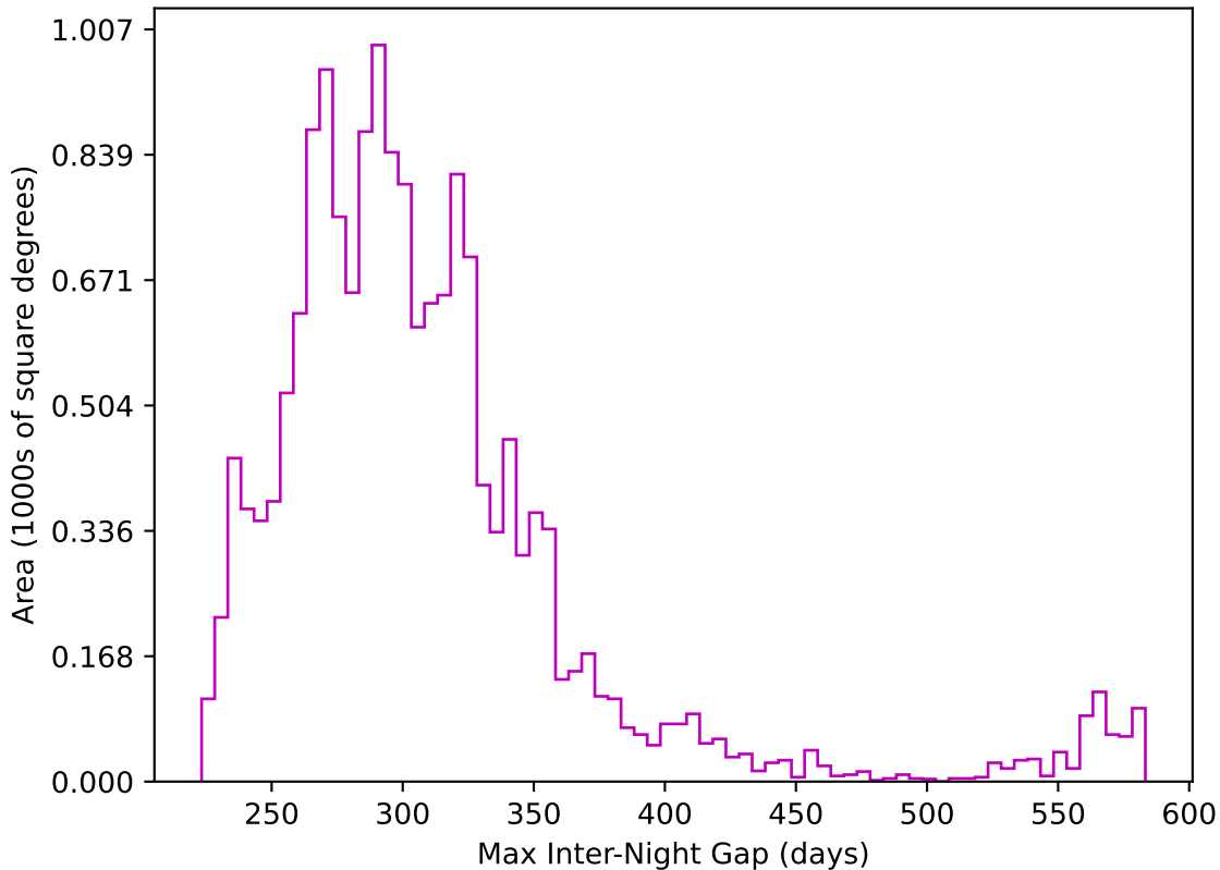
too_elab_r256_d3_giz_v3.4_10yrs WFD z band: Max Inter-Night Gap
