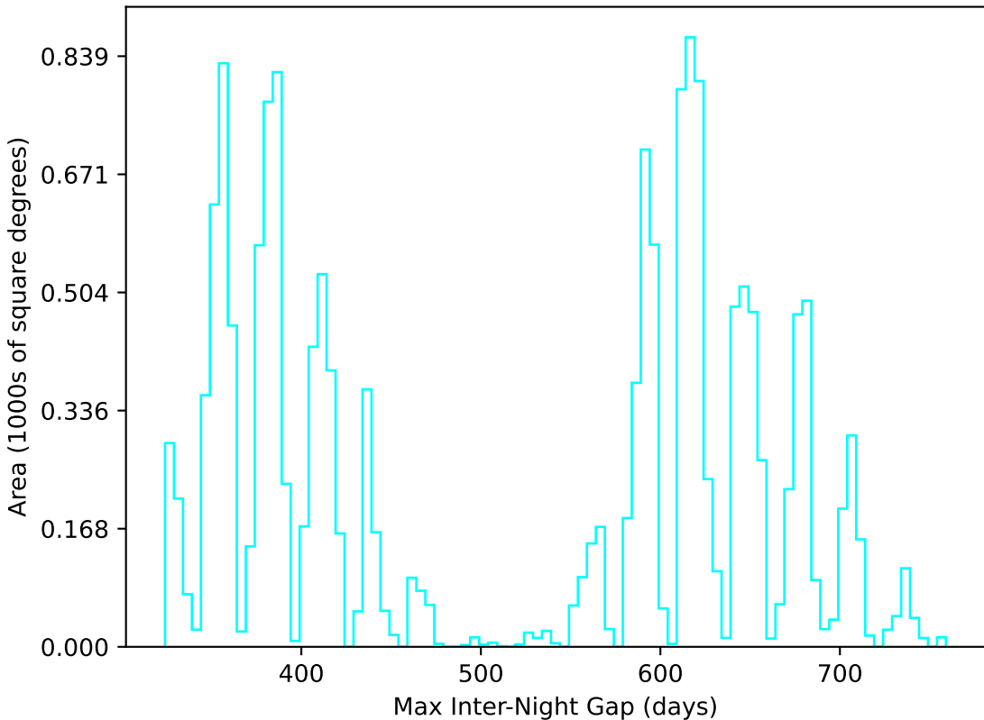
too_elab_r256_d3_giz_v3.4_10yrs WFD u band: Max Inter-Night Gap
