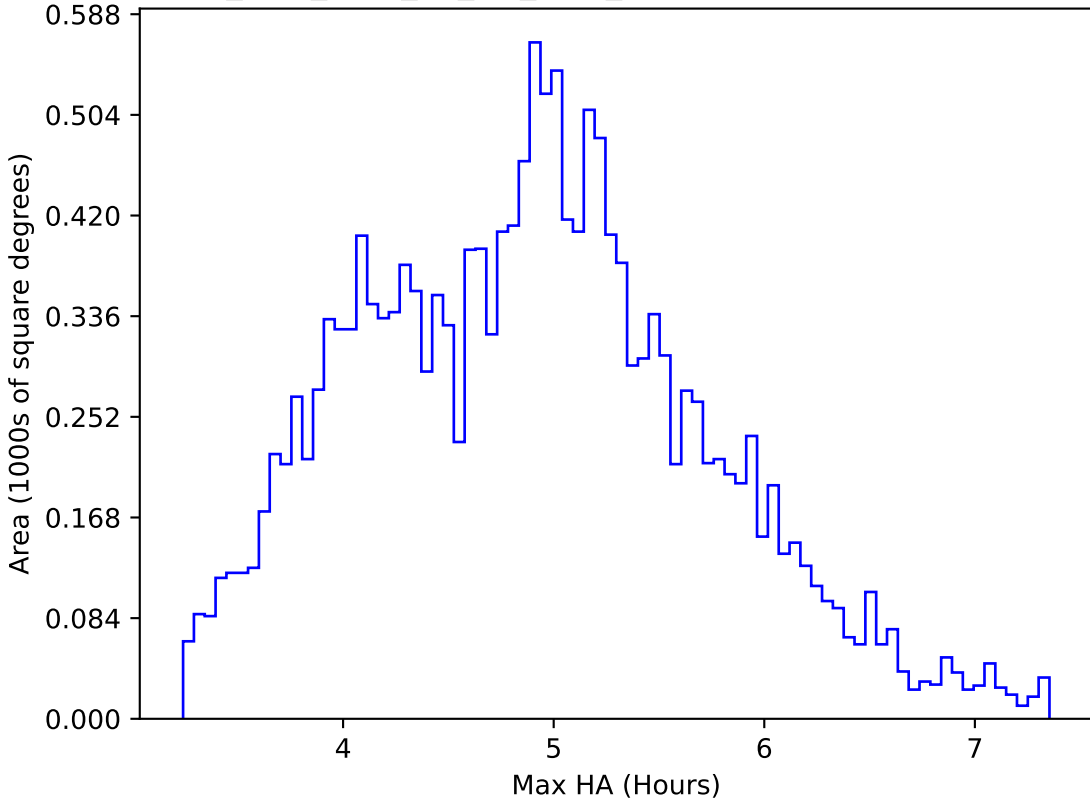
too_elab_r256_d3_giz_v3.4_10yrs WFD z band: Max HA
