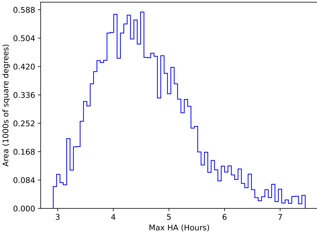
too_elab_r256_d3_giz_v3.4_10yrs WFD r band: Max HA
