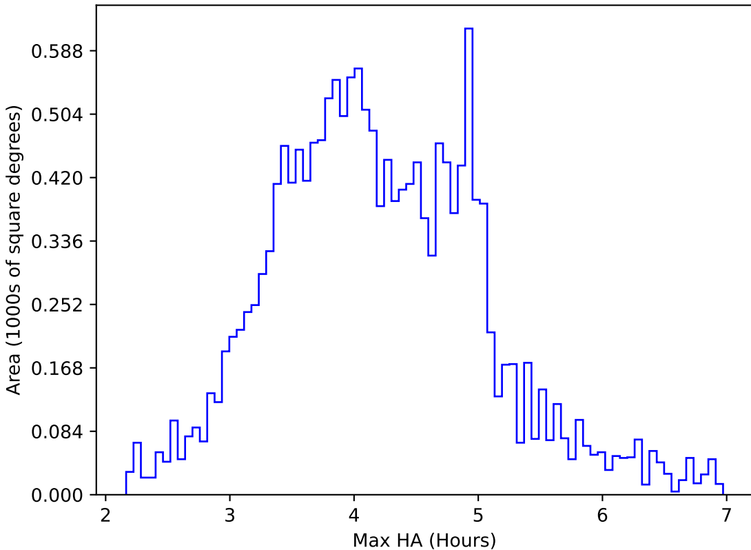
too_elab_r256_d3_giz_v3.4_10yrs WFD g band: Max HA
