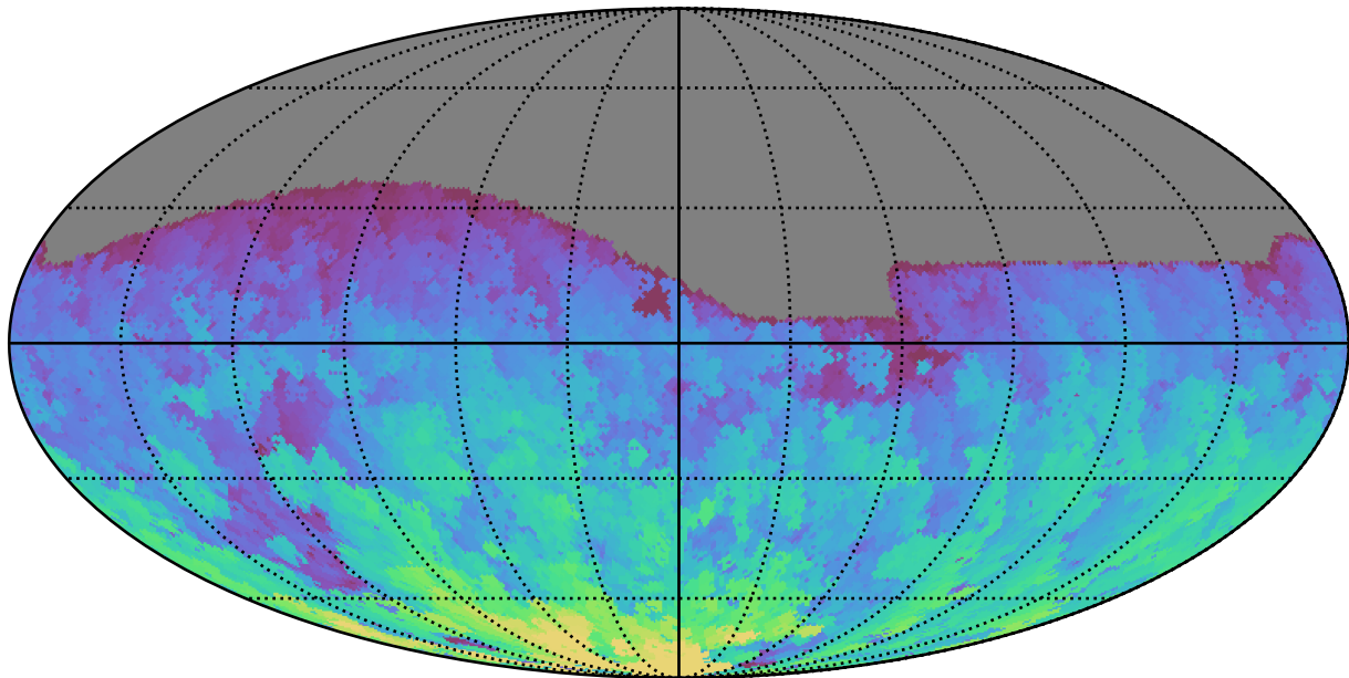
too_elab_r256_d3_giz_v3.4_10yrs All sky g band: Max HA
