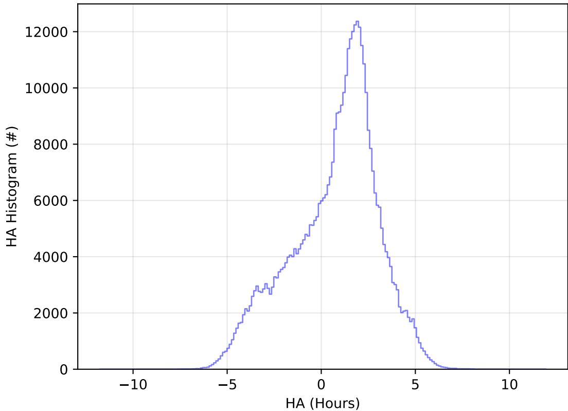
too_elab_r256_d3_giz_v3.4_10yrs WFD z band: HA Histogram
