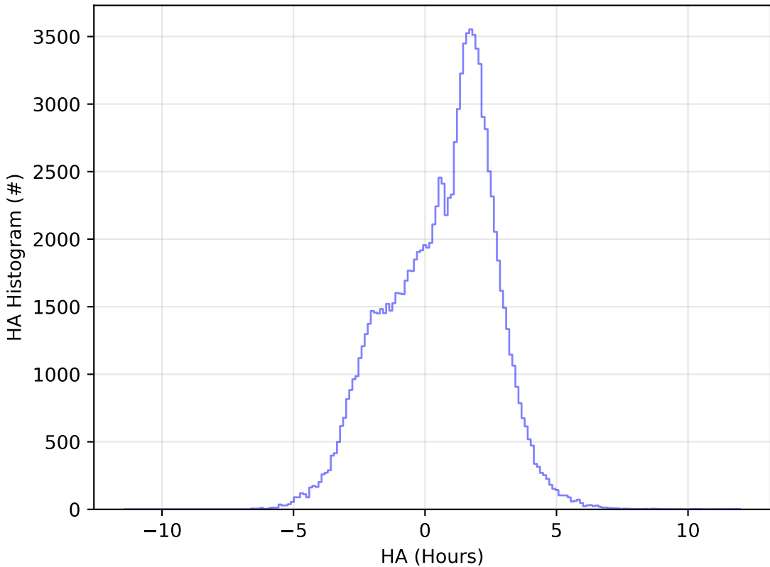
too_elab_r256_d3_giz_v3.4_10yrs WFD u band: HA Histogram
