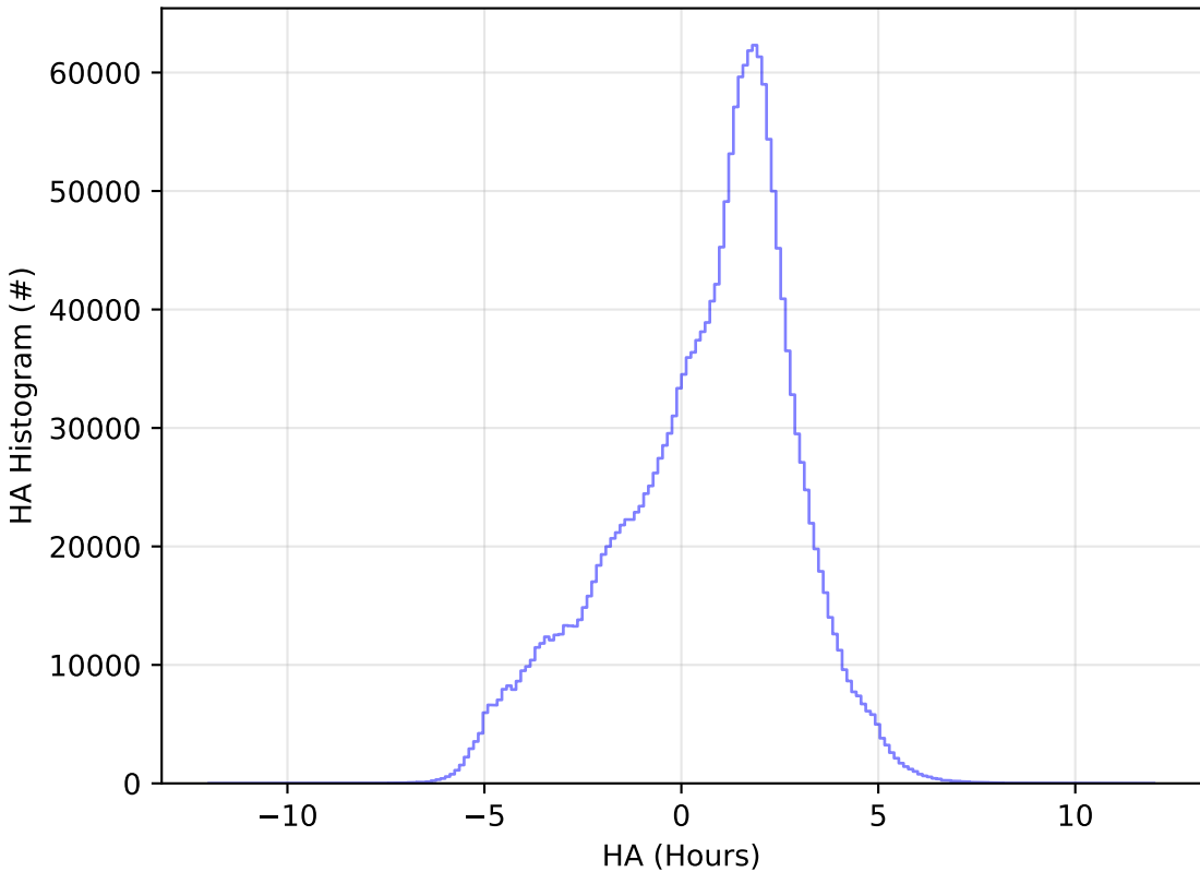
too_elab_r256_d3_giz_v3.4_10yrs WFD all bands: HA Histogram
