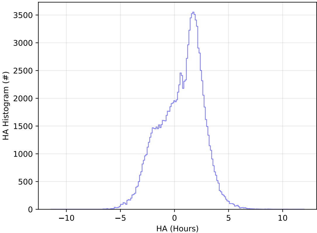
too_elab_r256_d3_giz_v3.4_10yrs All sky u band: HA Histogram
