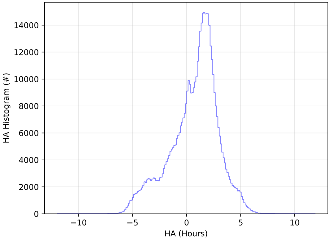
too_elab_r256_d3_giz_v3.4_10yrs All sky i band: HA Histogram
