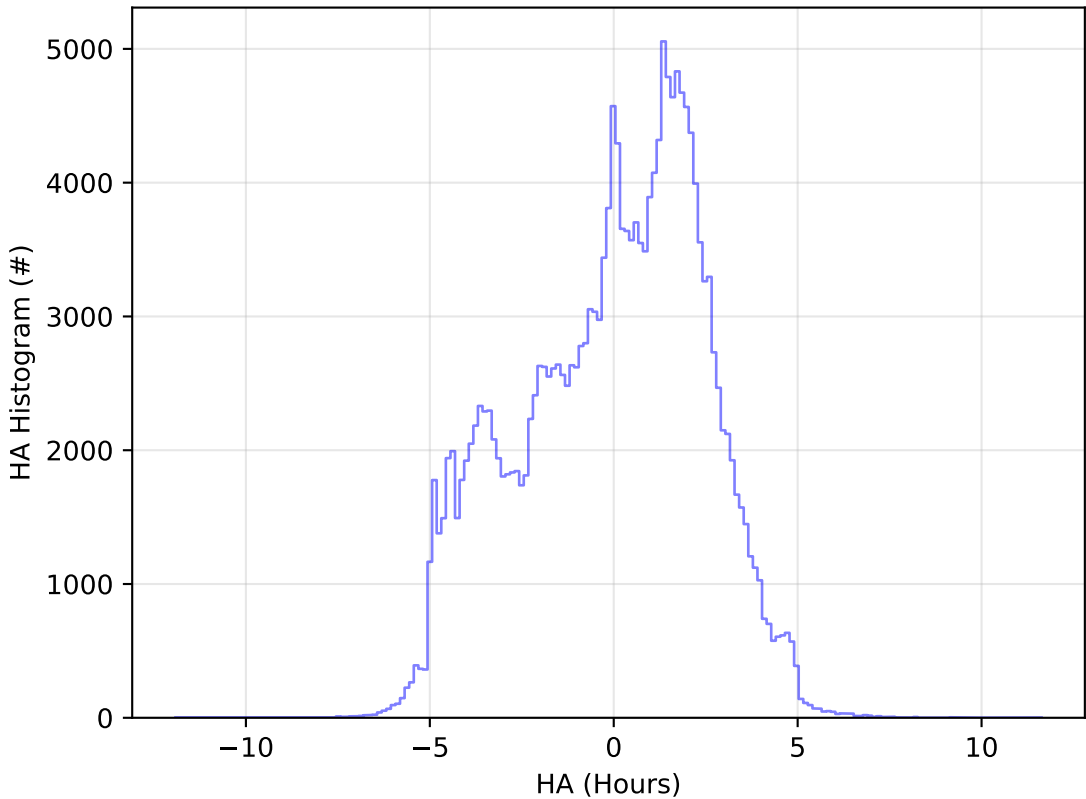
too_elab_r256_d3_giz_v3.4_10yrs All sky g band: HA Histogram
