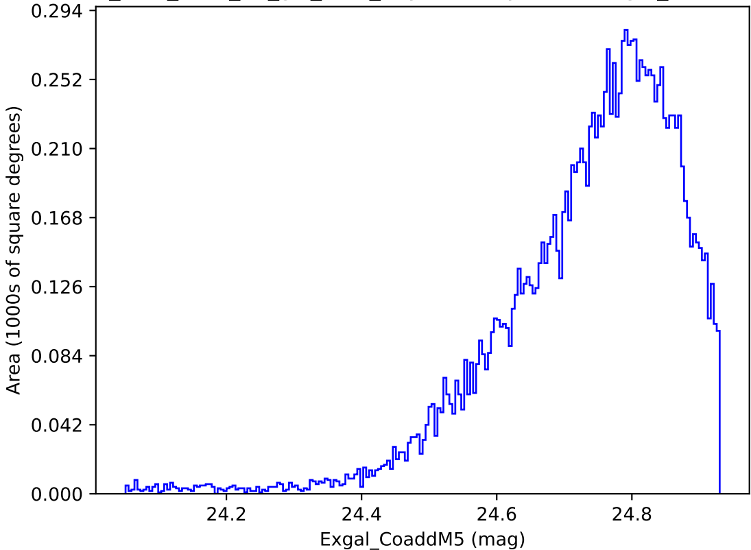
too_elab_r256_d3_giz_v3.4_10yrs WFD y band: Exgal_CoaddM5
